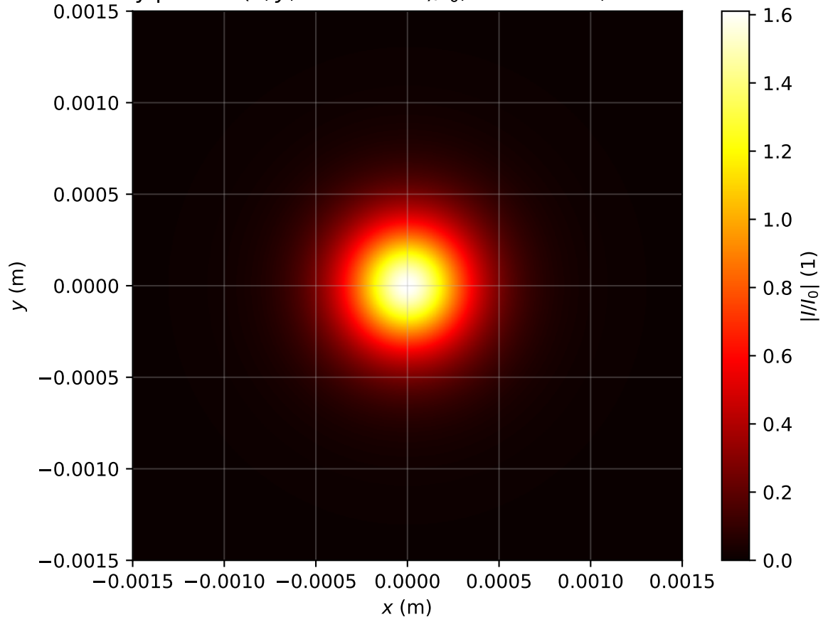
Intensity profile I(x, y, z = 2.627m)/I_0 , Pin=0.9Pcr, artificial time
